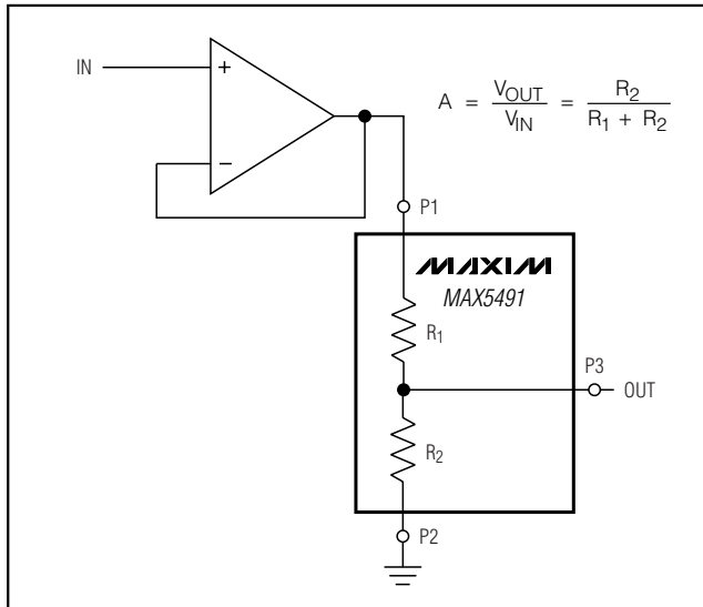
Figure 3. Buffered Attenuator
