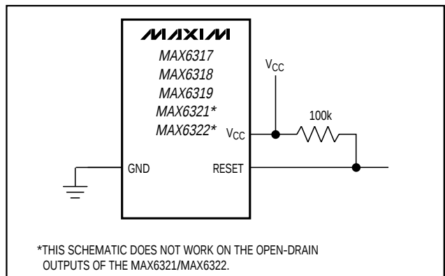
Figure 9. Ensuring RESET Valid to V_{CC} = 0 on Active-High Push/Pull Outputs
