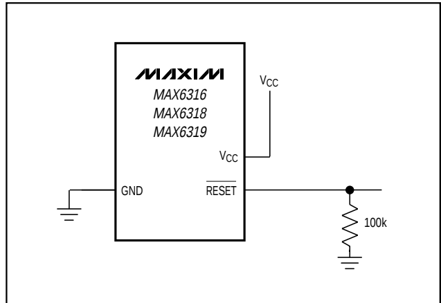
Figure 8. Ensuring \overline{RESET} Valid to V_{CC} = 0 on Active-Low Push/Pull and Bidirectional Outputs
