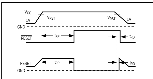
Figure 2. Reset Timing Diagram
