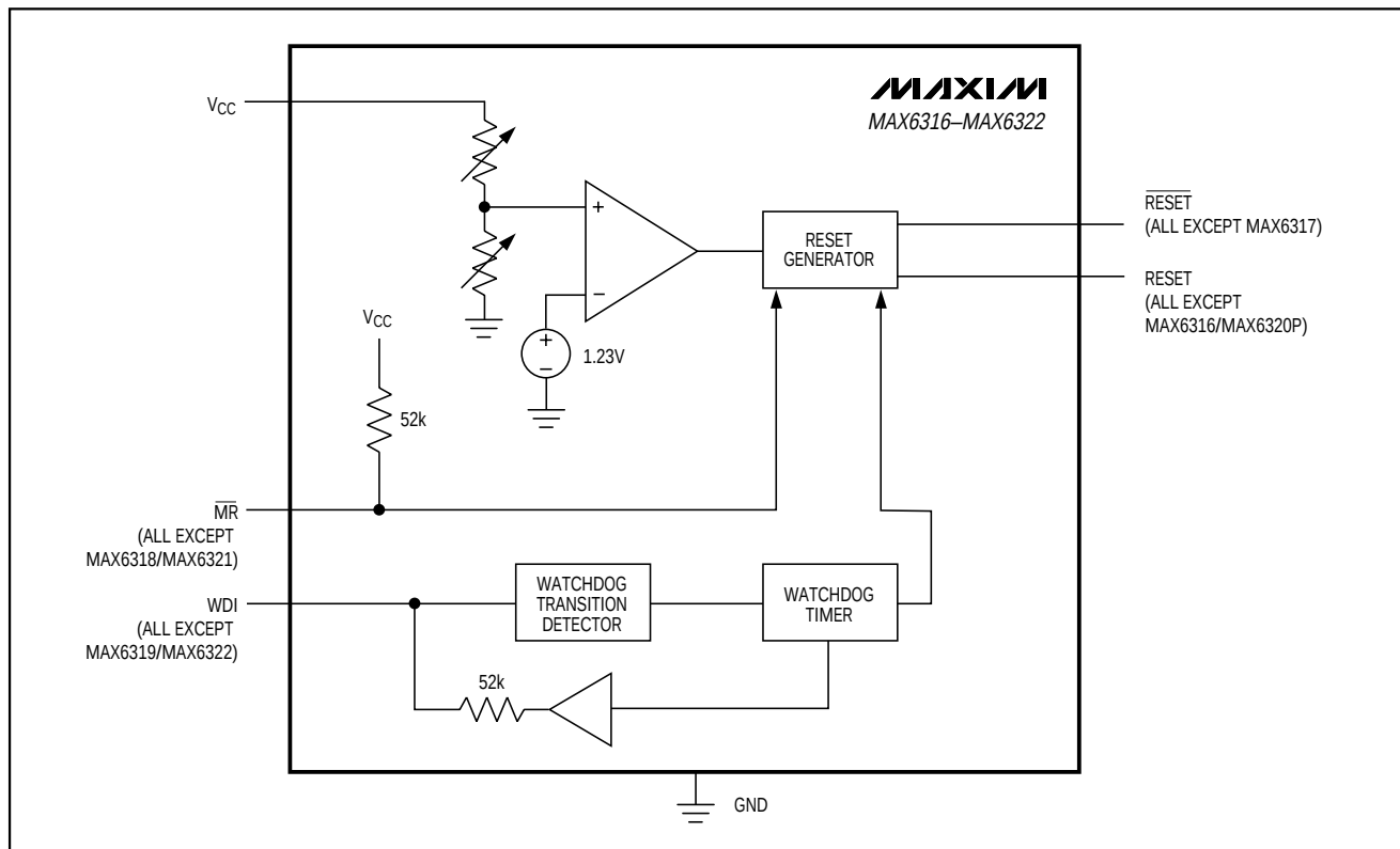
Figure 1. Functional Diagram
