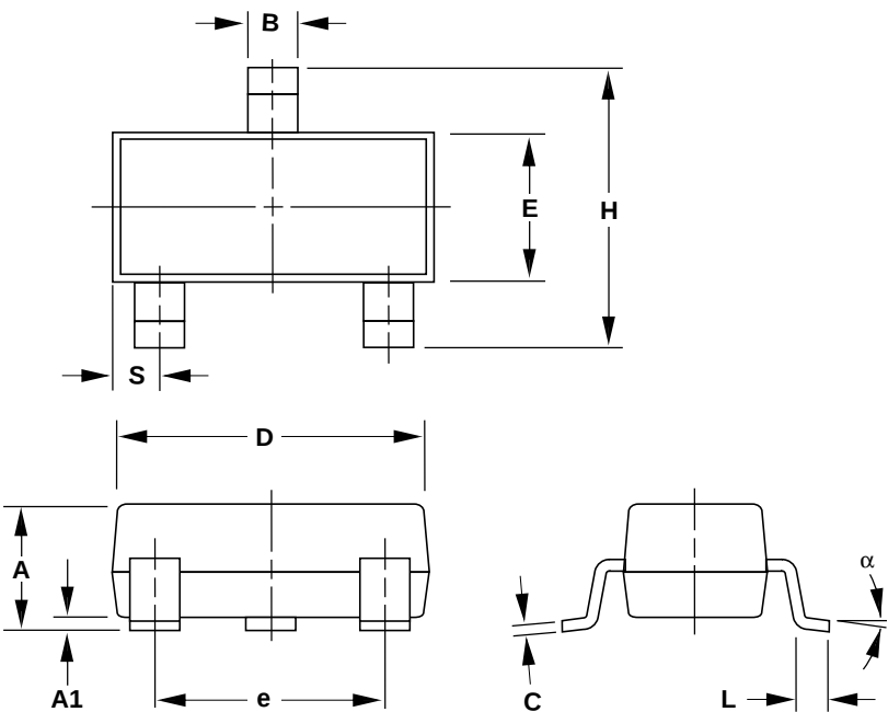
3-PIN SOT23-3 SMALL-OUTLINE TRANSISTOR PACKAGE
