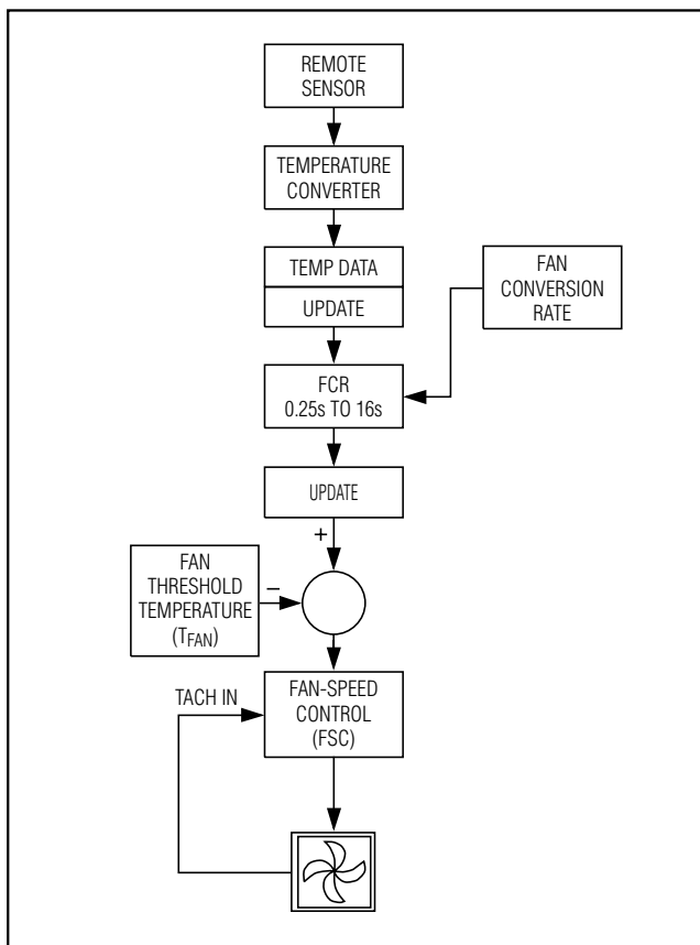
Figure 6. MAX6661 Thermal Loop
