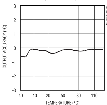
OUTPUT ACCURACY vs. TEMPERATURE
