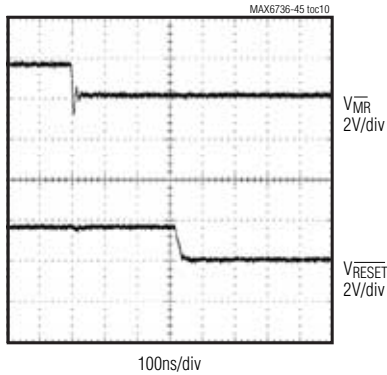
\overline{\text{MR}} TO RESET OUTPUT DELAY
