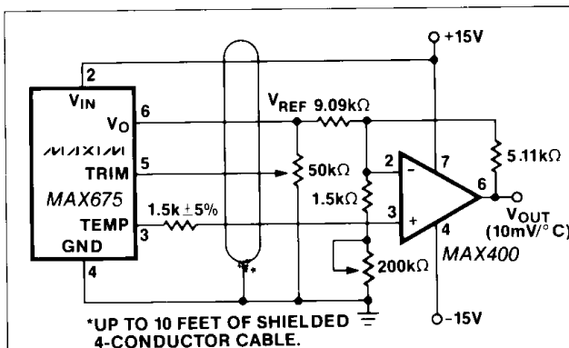
Figure 6. Precision Temperature Transducer with Remote Sensor
