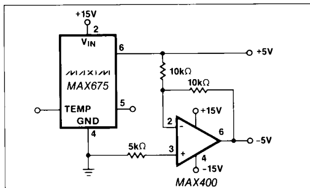
Figure 4. +5V Reference
