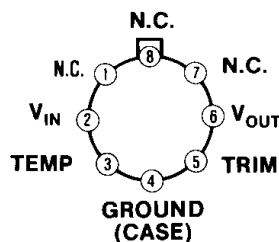
TO-99 Metal Can
