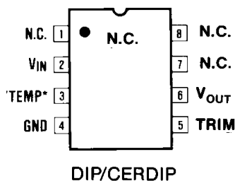
DIP/CERDIP
