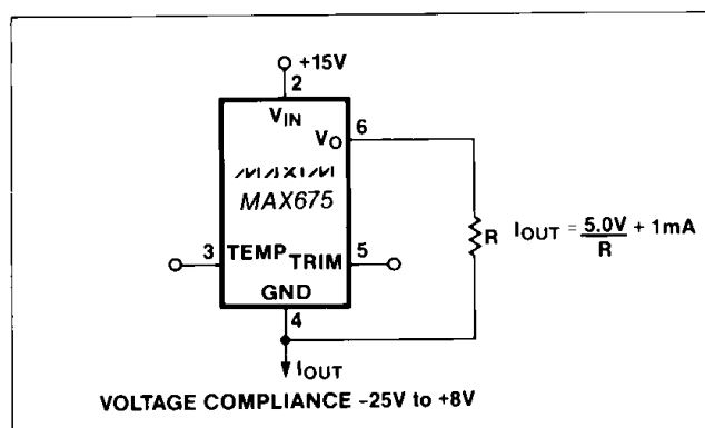
Figure 5. Current Source
