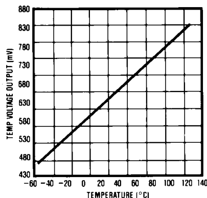
Figure 2. MAX675 Temperature Voltage Output vs. Temperature
