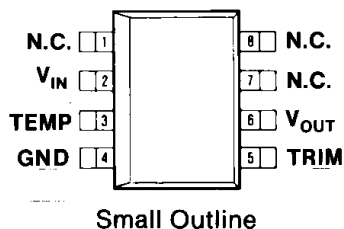
Small Outline
