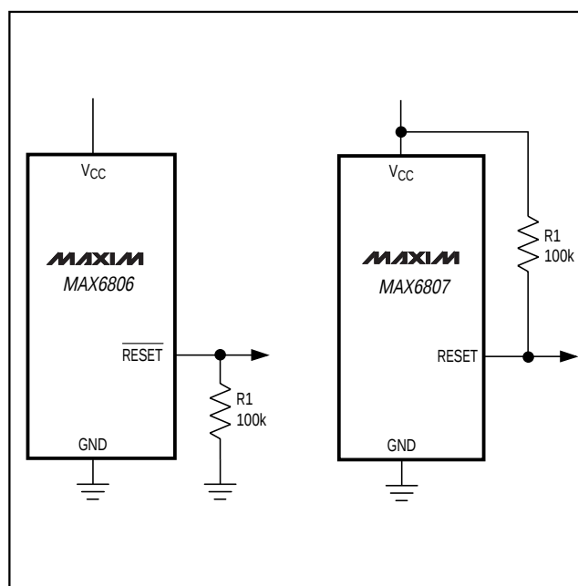
Figure 4. \overline{RESET} / RESET Valid to VCC = Ground Circuit
