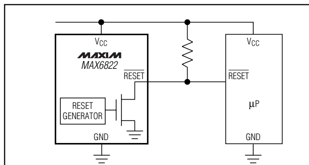
Figure 4. Interfacing Open-Drain \overline{\text{RESET}} to \mu Ps with Bidirectional Reset I/O
