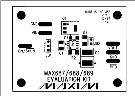
Figure 2. MAX688 EV Kit Component Placement Guide—Component Side
