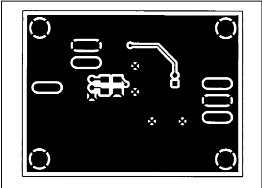
Figure 5. MAX688 EV Kit PC Board Layout—Solder Side
