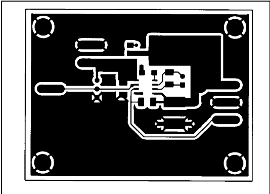
Figure 4. MAX688 EV Kit PC Board Layout—Component Side
