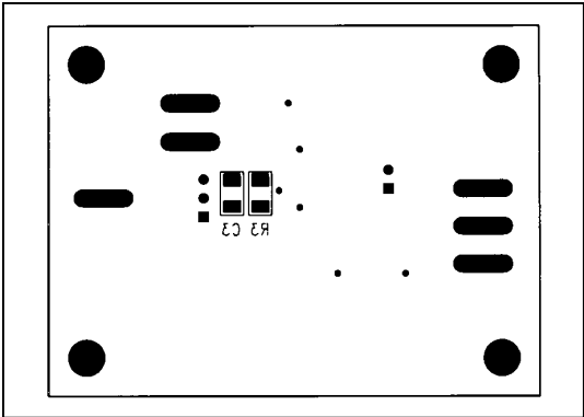
Figure 3. MAX688 EV Kit Component Placement Guide—Solder Side
