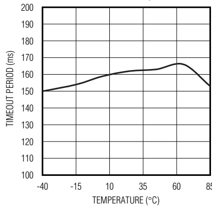
RESET TIMEOUT PERIOD vs. TEMPERATURE ( C_{RST} = 0.047\mu\text{F} )
