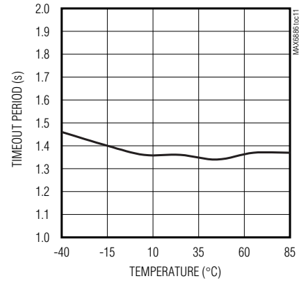
WATCHDOG TIMEOUT PERIOD vs. TEMPERATURE ( C_{SWT} = 0.33\mu\text{F} )
