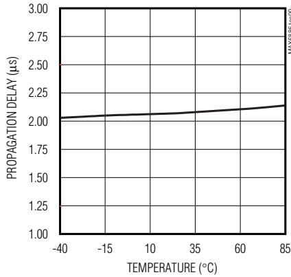
\overline{\text{MR}} TO RESET OUTPUT PROPAGATION DELAY vs. TEMPERATURE
