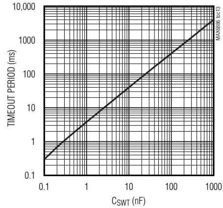
WATCHDOG TIMEOUT PERIOD vs. C_{SWT}
