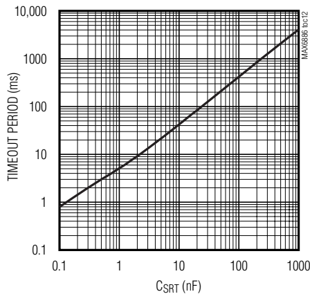
RESET TIMEOUT PERIOD vs. C_{RST}
