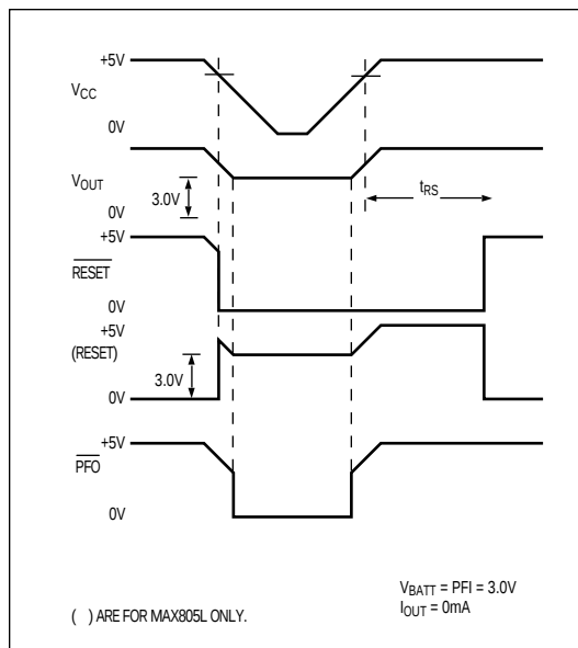
Figure 2. Timing Diagram
