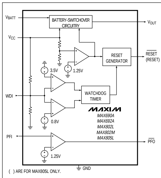
Figure 1. Block Diagram
