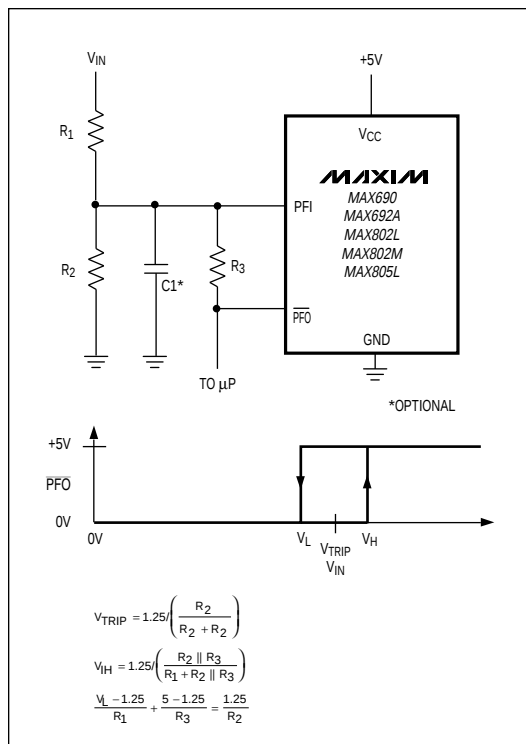
Figure 6. Adding Hysteresis to the Power-Fail Comparator
