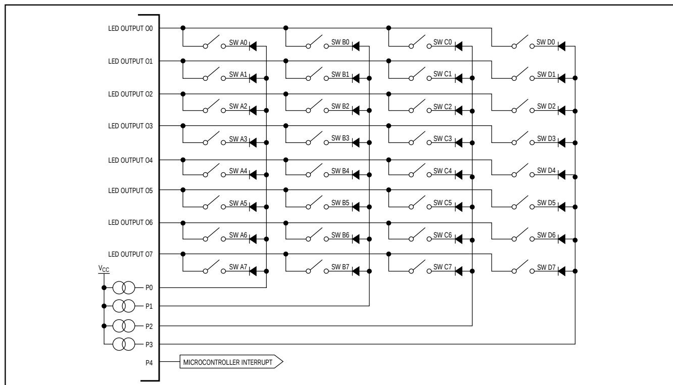
Figure 7. Key-Scanning Configuration
