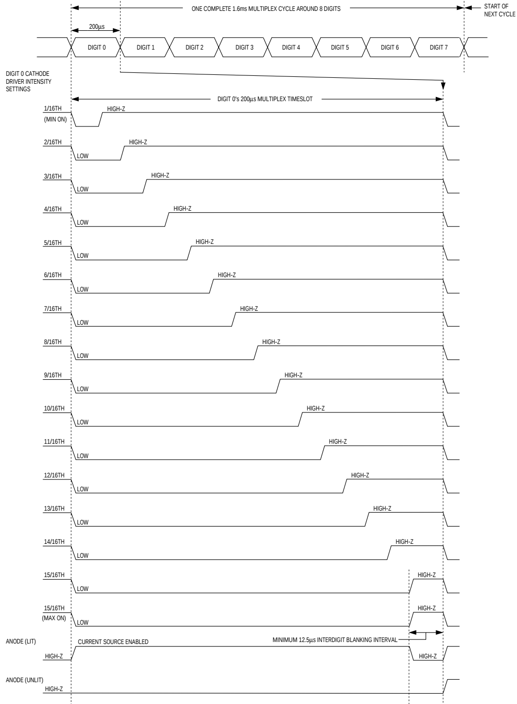
Figure 6. Multiplex Timing Diagram (OSC = 4MHz)
