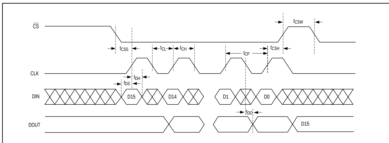
Figure 3. Timing Diagram
