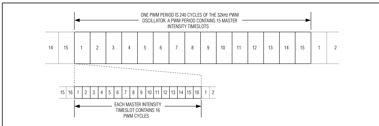
Figure 12. PWM Timing
