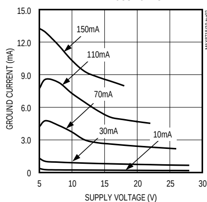
GROUND CURRENT vs. SUPPLY VOLTAGE AT VARIOUS LOADS
