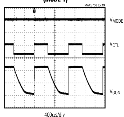
HIGH-VOLTAGE SWITCH CONTROL FUNCTION (MODE 1)
