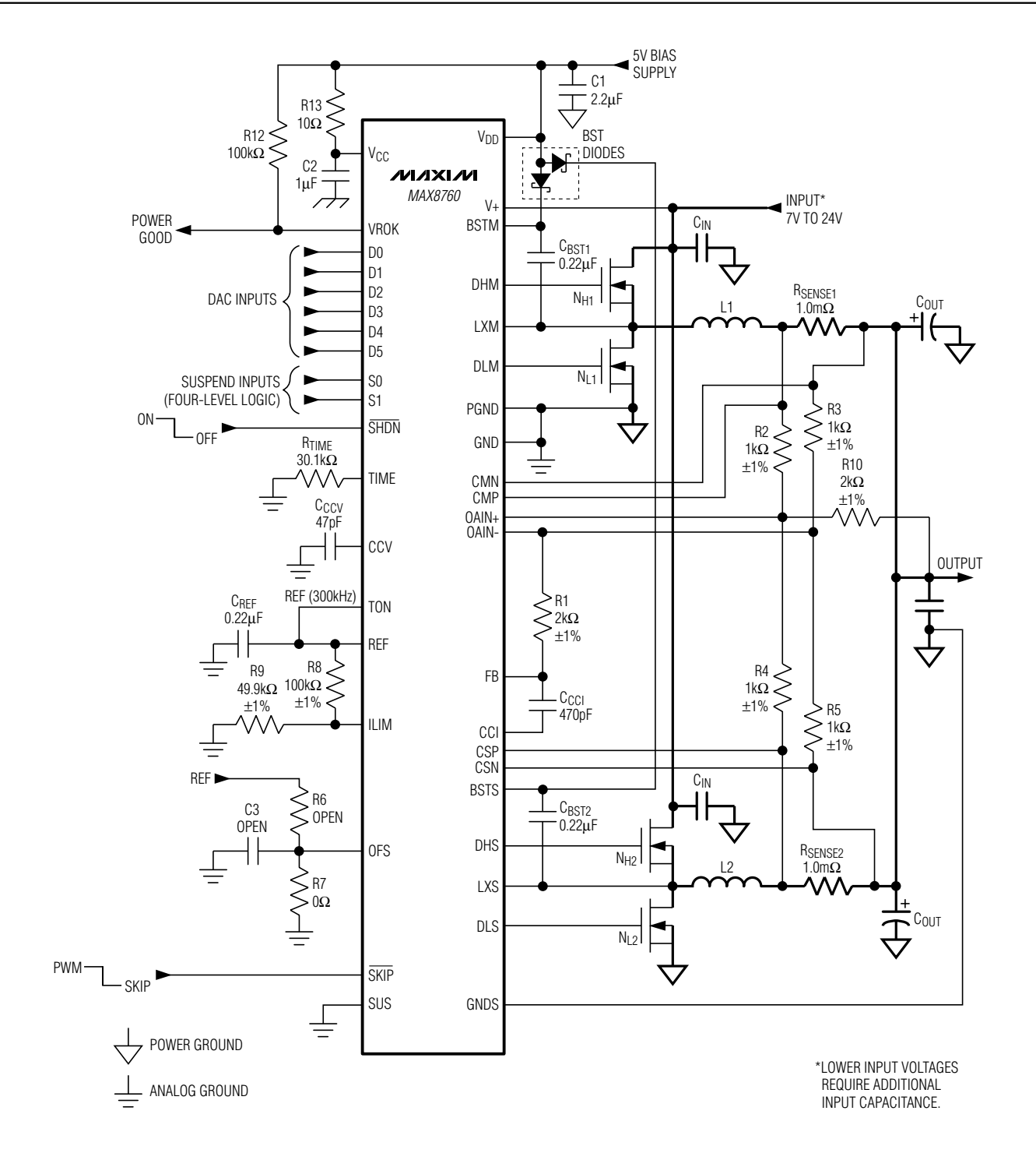
Figure 1. Standard Two-Phase AMD Mobile 30A Application Circuit
