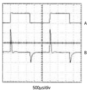
LINE-TRANSIENT RESPONSE
