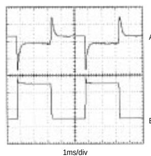
LOAD-TRANSIENT RESPONSE
