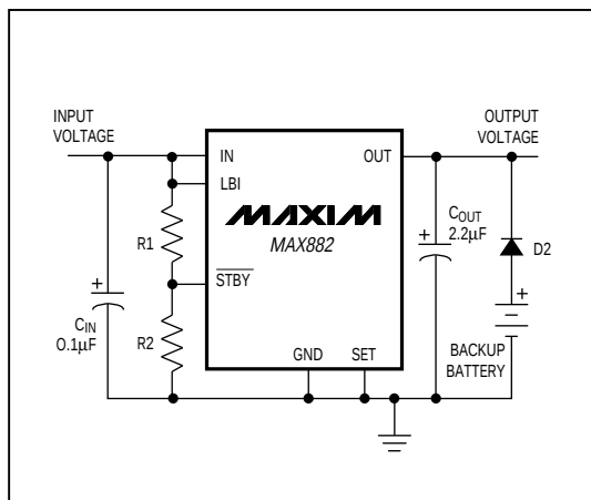
Figure 9. Short-Term Battery Backup Using the MAX882
