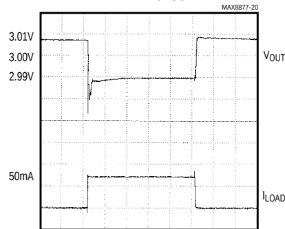
LOAD-TRANSIENT RESPONSE NEAR DROPOUT
