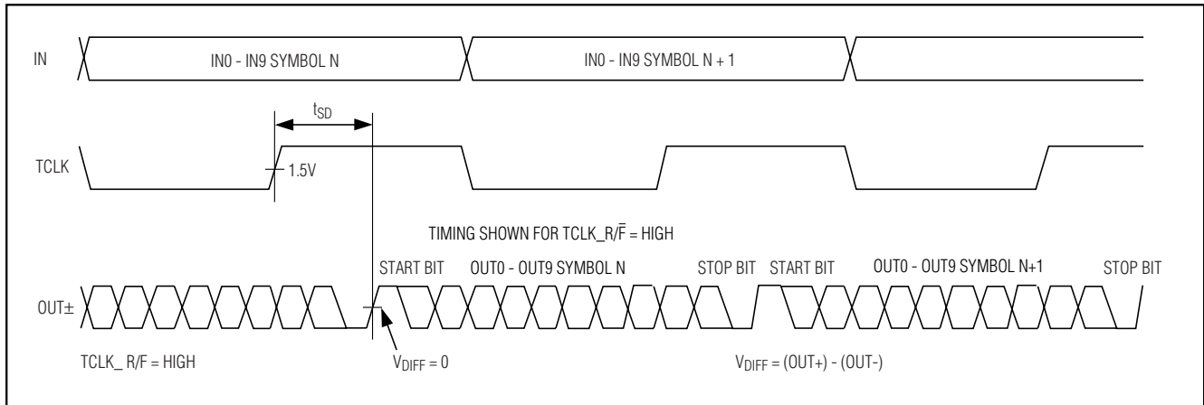
Figure 8. Serializer Delay
