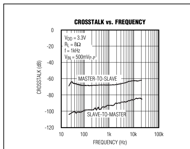
Figure 9. Master-Slave Crosstalk
