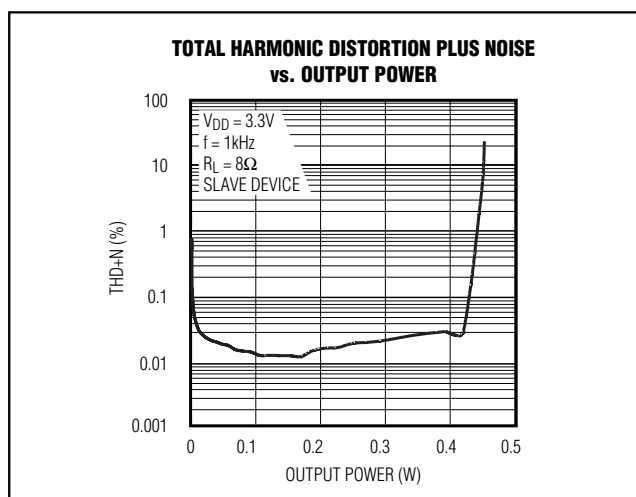
Figure 8. Master-Slave THD+N
