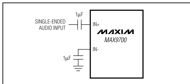
Figure 6. Single-Ended Input
