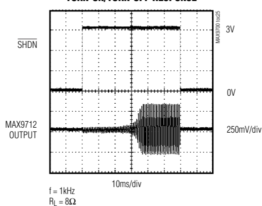
TURN-ON/TURN-OFF RESPONSE
