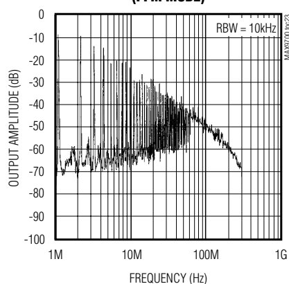
WIDEBAND OUTPUT SPECTRUM (FFM MODE)
