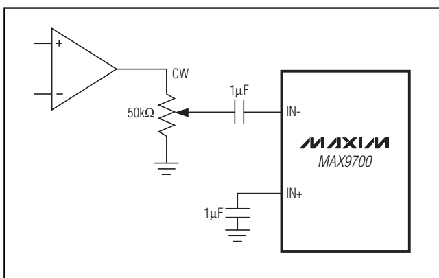
Figure 10a. Single-Ended Drive of MAX9700 Plus Volume
