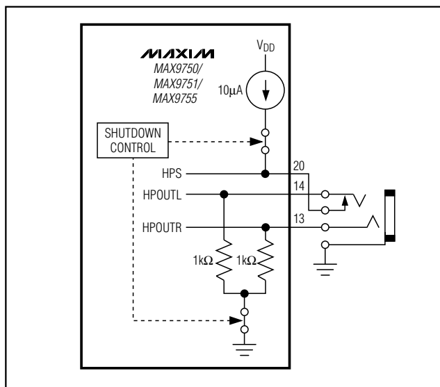
Figure 5. HPS Configuration
