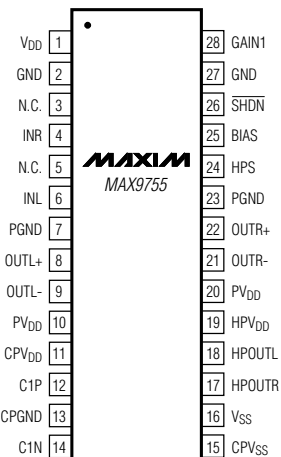
TSSOP-EP
