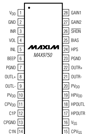
TSSOP-EP
