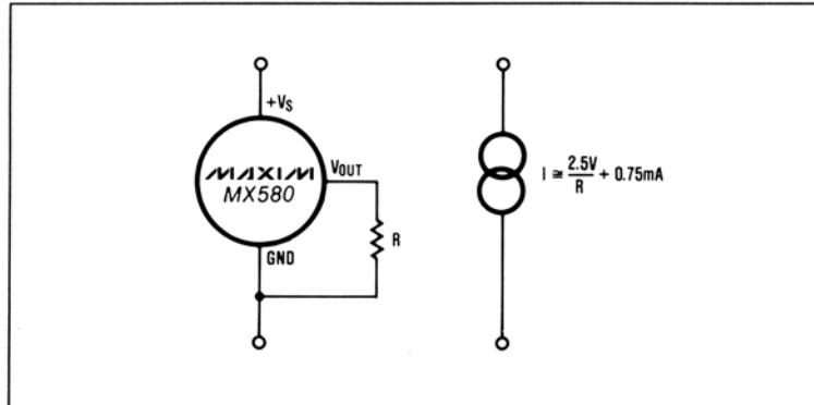
Figure 1. Two-Component Precision Current Limiter
