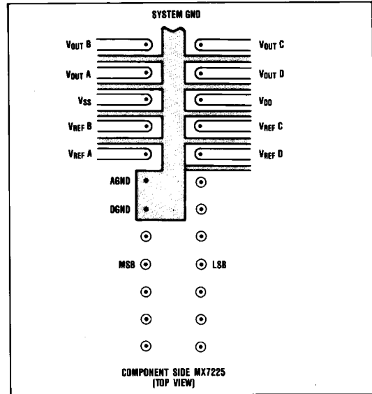
Figure 8. Suggested MX7225 PCB Layout for Minimizing Crosstalk
