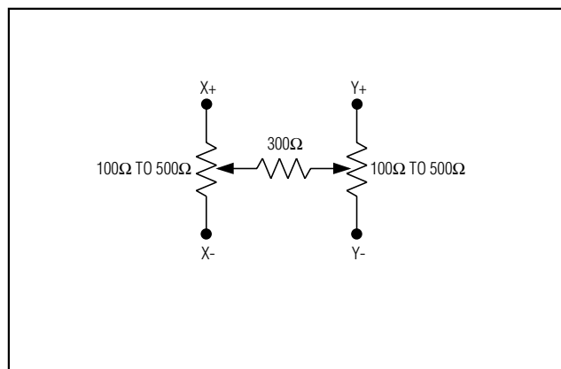
Figure 6. Touch-Screen Equivalent Circuit
