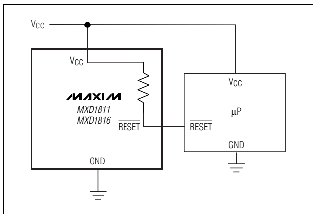
Figure 7. Interfacing to Microprocessors with Bidirectional Reset Pins
