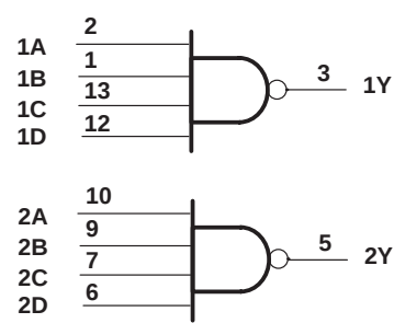
logic diagram (positive logic)
