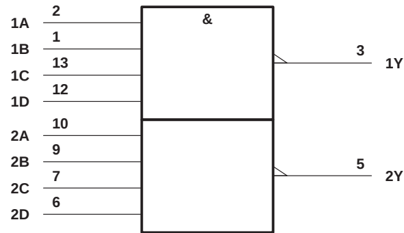
logic symbol†
