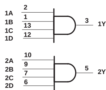
logic diagram (positive logic)
