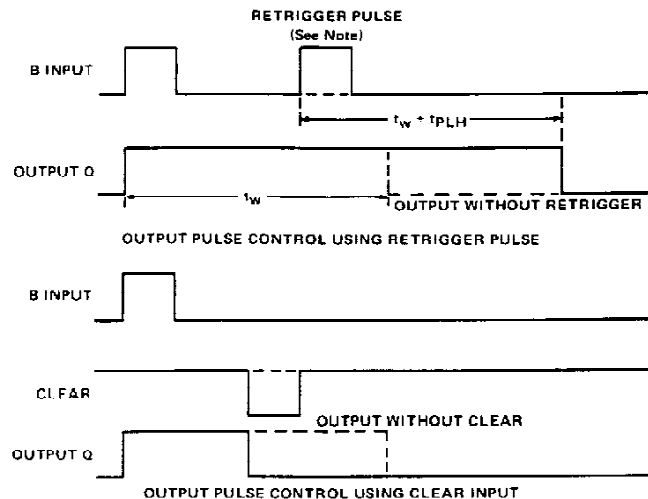
FIGURE 1—TYPICAL INPUT/OUTPUT PULSES
