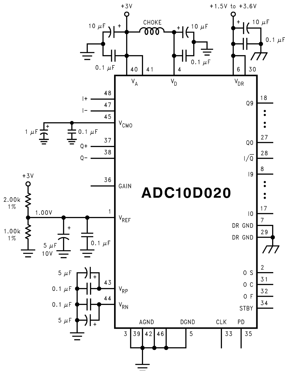
Figure 64. Simple Reference Biasing
