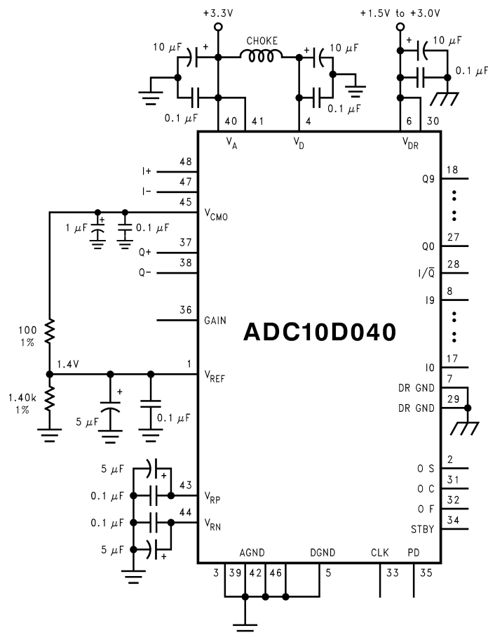
Figure 37. The V_{CMO} output pin may be used as an internal reference source if its output is not loaded excessively.
