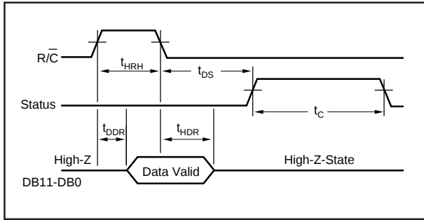
FIGURE 4. \overline{R/C} Pulse High — Outputs Enabled Only While \overline{R/C} Is High.
