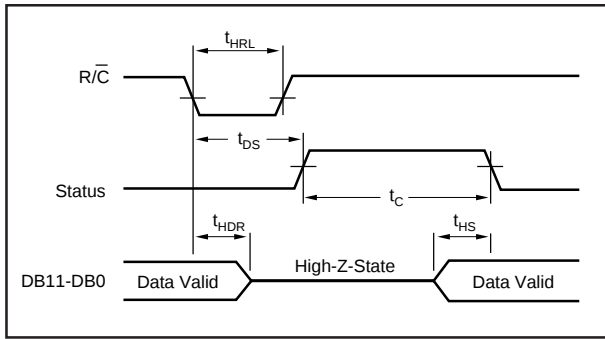
FIGURE 3. \overline{R/C} Pulse Low—Outputs Enabled After Conversion.
