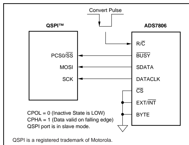
FIGURE 12. QSPI Interface to the ADS7806.
