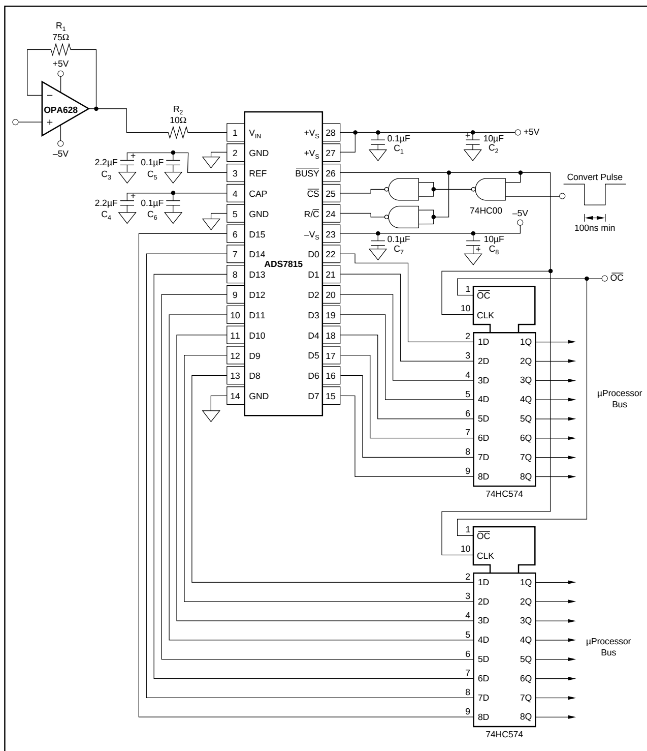
FIGURE 1. Basic Operation.
