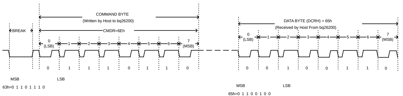
Figure 4. Communication Sequence
