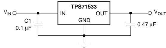
Figure 13. Typical Application Circuit (Fixed Voltage Version)
