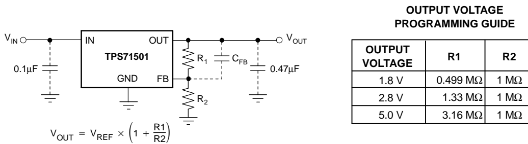
Figure 14. TPS71501 Adjustable LDO Regulator Programming
