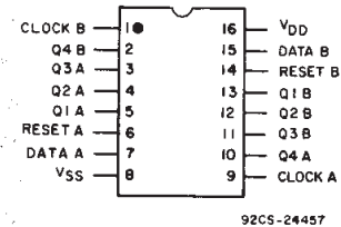
TERMINAL DIAGRAM
