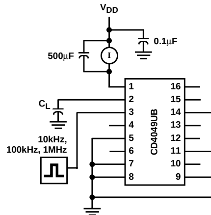
FIGURE 17. DYNAMIC POWER DISSIPATION TEST CIRCUITS
