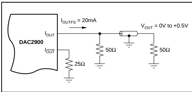
FIGURE 6. Driving a Doubly Terminated 50Ω Cable Directly.
