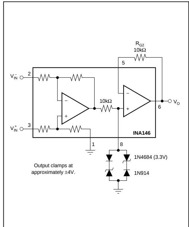
FIGURE 5. Output Clamp.
