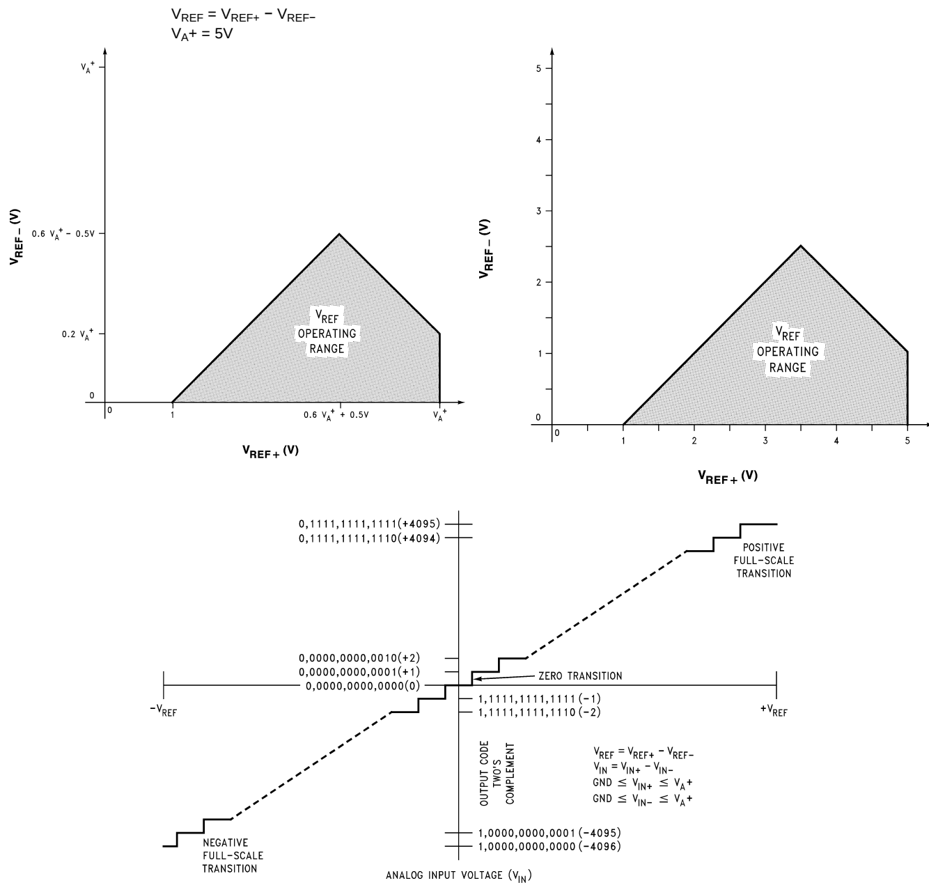
Figure 4. Transfer Characteristic
