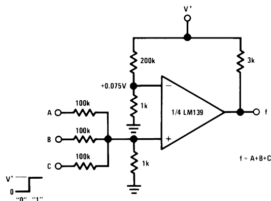
Figure 17. OR Gate
