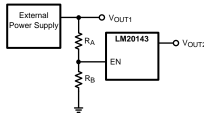
Figure 33. Sequencing LM20143 with Precision Enable
