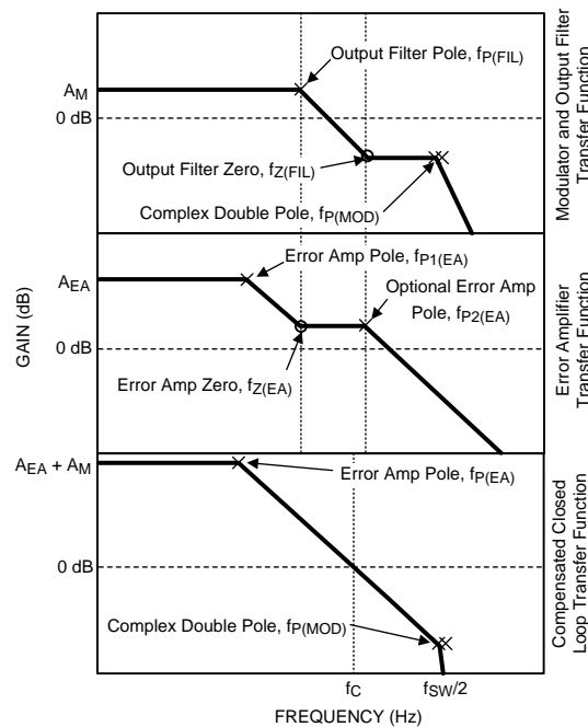
Figure 31. LM20143 Loop Compensation
