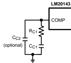
Figure 32. Compensation Network for LM20143
