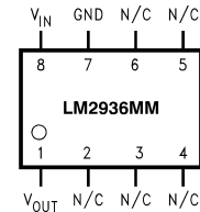
Figure 4. 8-Pin VSSOP (MM) Top View
