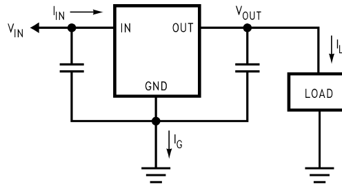
Figure 24. Power Dissipation Diagram
