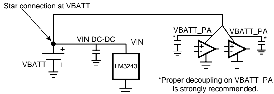
Figure 33. VBATT Star Connection on VIN and VBATT_PA
