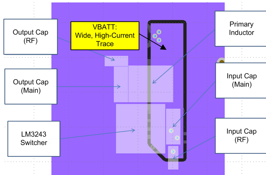
Figure 31. Board Layer 5 - VBATT_SW Connection
