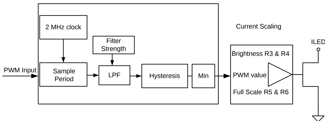
Figure 86. PWM Sampler
