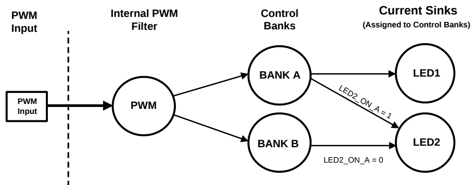
Figure 74. Control Diagram
