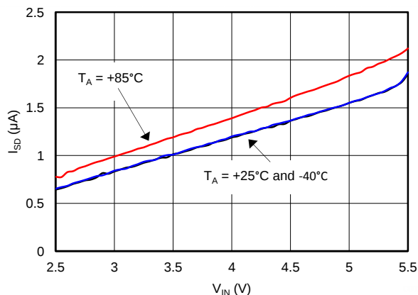
Figure 37. Shutdown Current vs. V_{IN} EN = 0\text{V}
